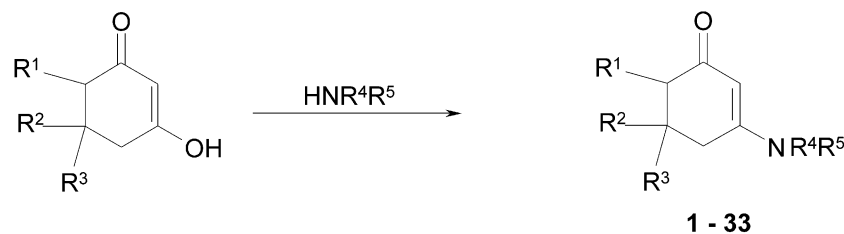
Scheme 1. General scheme for the synthesis of cyclic enaminones.
