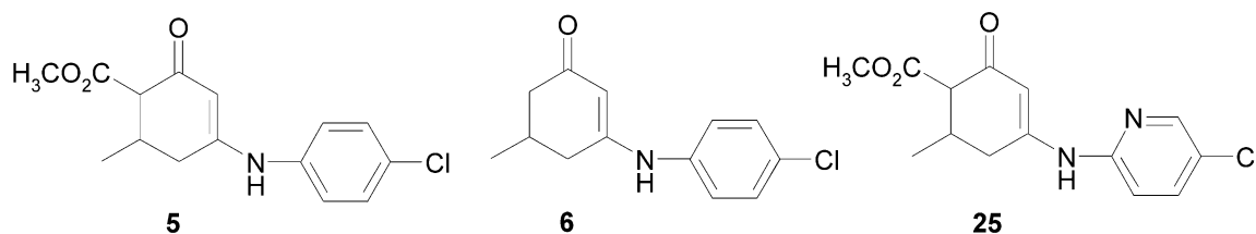
Scheme 2. Structures of potent anticonvulsant enaminones 5 , 6 , and 25 .
